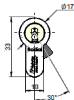
Cylindre double
